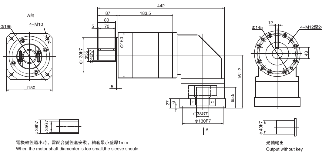
WPLR160三級 / Three stage
