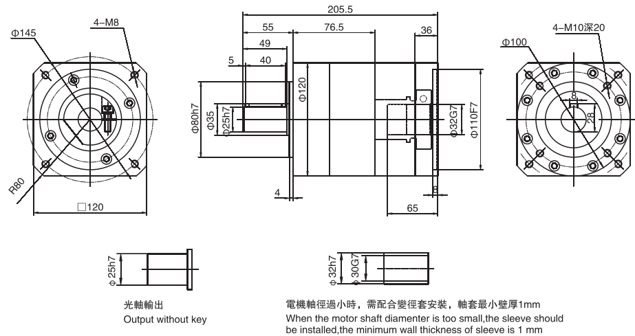
WPL120雙級 / Double stage
