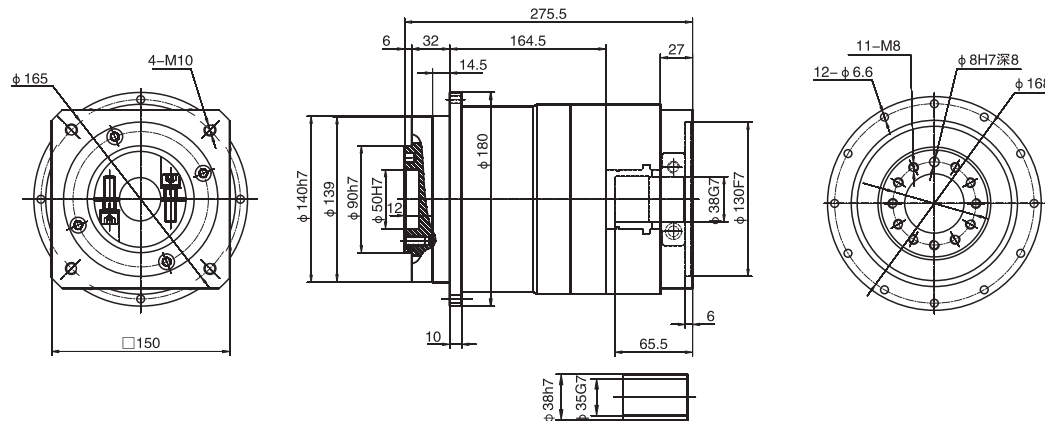
WPLH160三級 / Three stage
