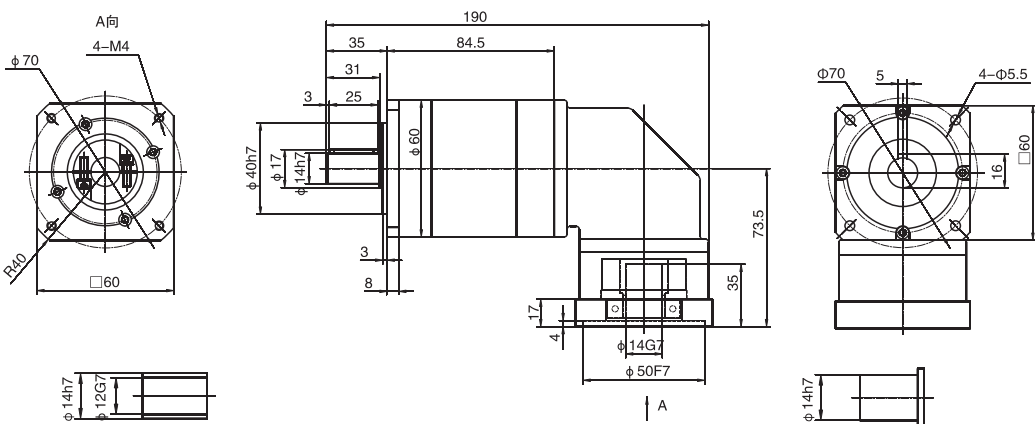
WPLFR60三級 / Three stage
