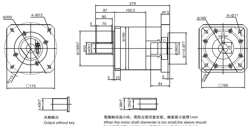
WPLF160單級 / Single stage
