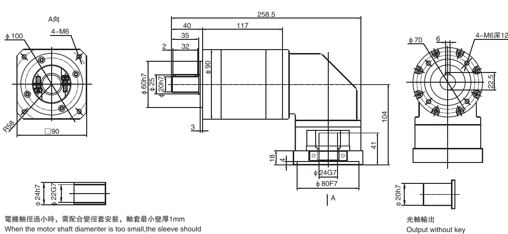
WPLR90三級 / Three stage
