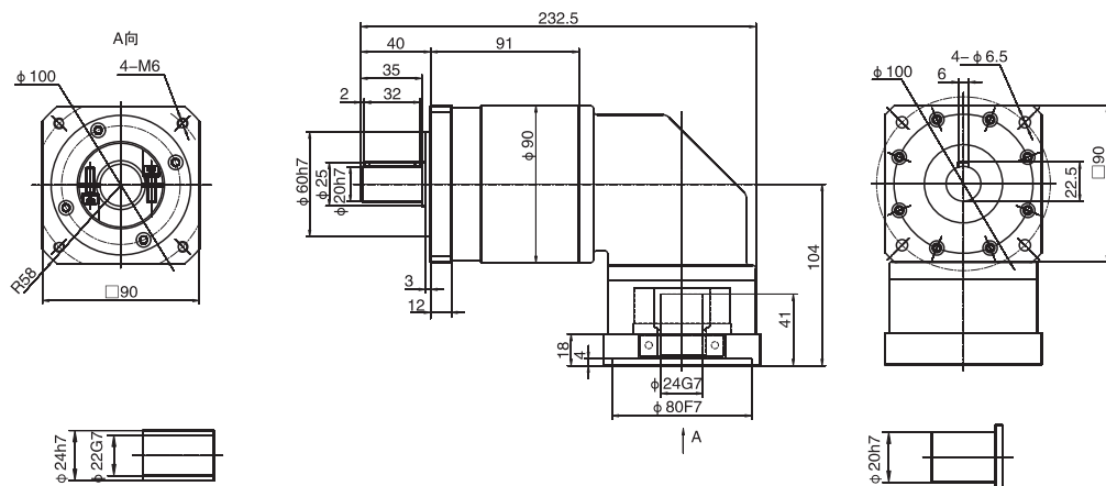
WPLFR90雙級 / Double stage
