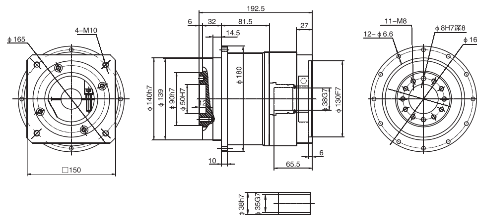
WPLH160單級 / Single stage
