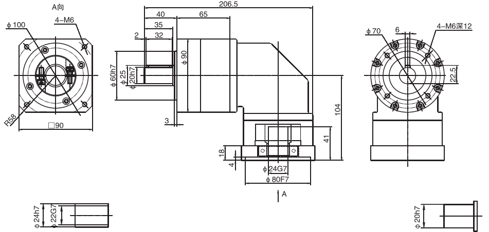
WPLR90單級 / Single stage
