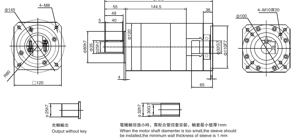
WPL120三級 / Three stage
