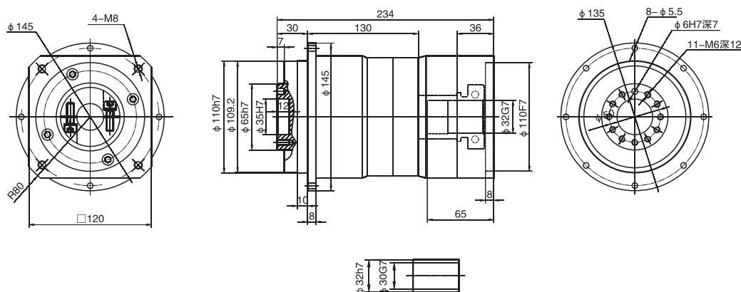
WPLH120三級 / Three stage
