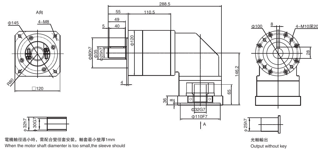
WPLR120雙級 / Double stage
