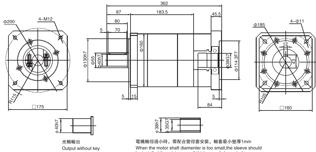
WPLF160三級 / Three stage
