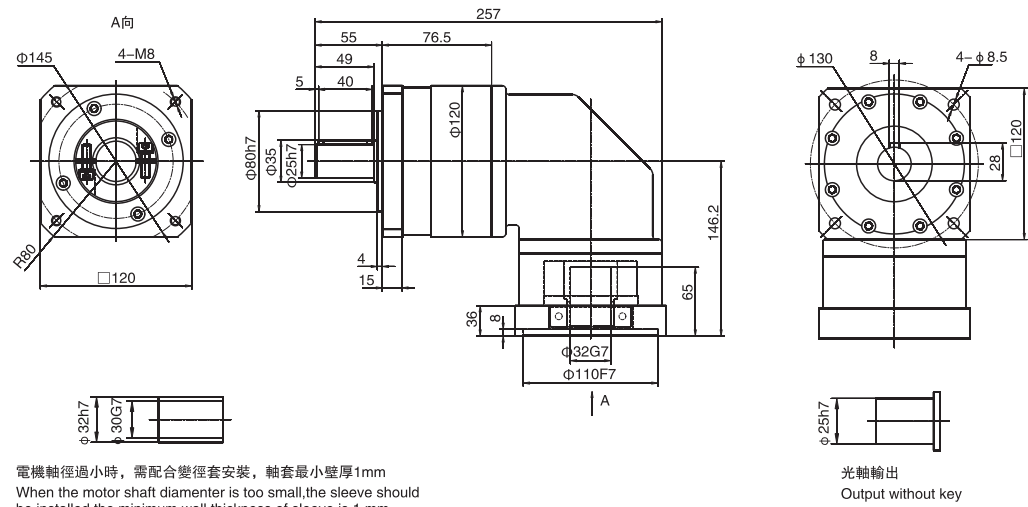
WPLFR120單級 / Single stage
