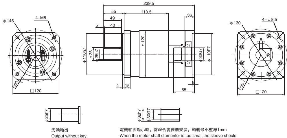
WPLF120雙級 / Double stage
