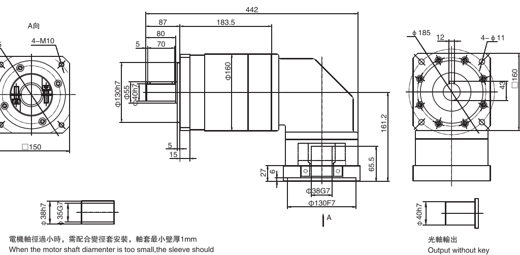
WPLFR160三級 / Three stage
