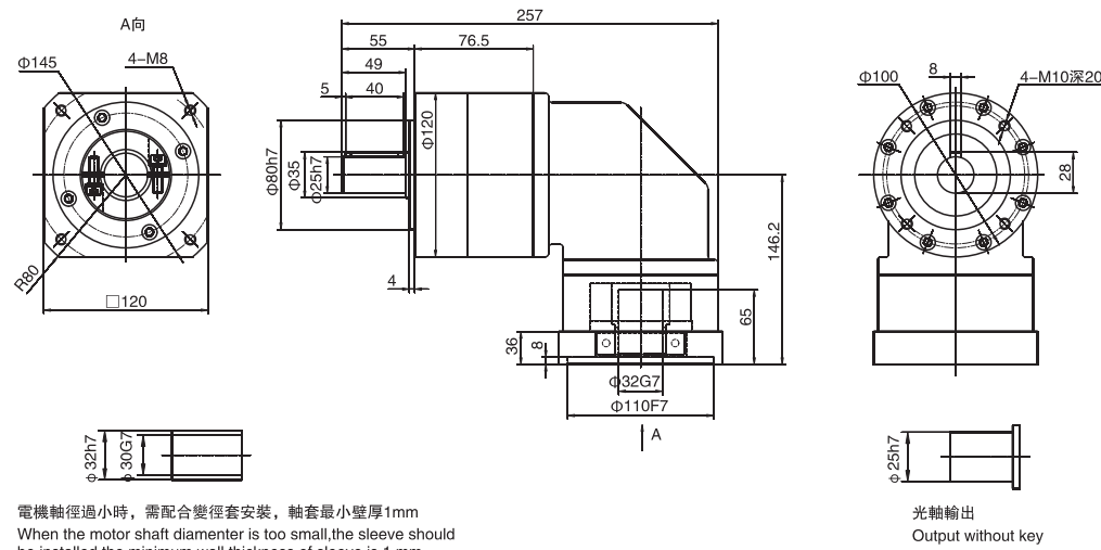
WPLR120單級 / Single stage
