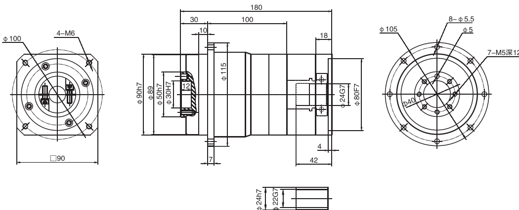
WPLH90三級 / Three stage
