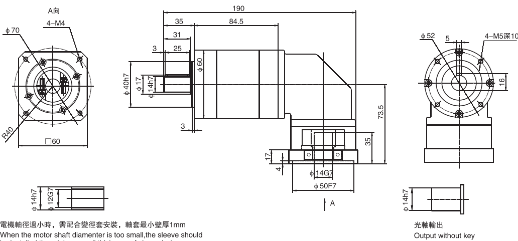
WPLR60三級 / Three stage
