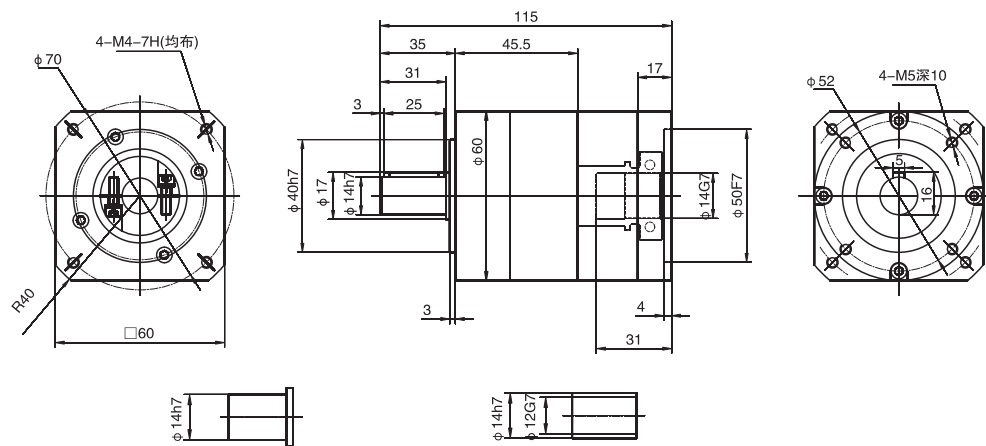
WPL60單級 / Single stage
