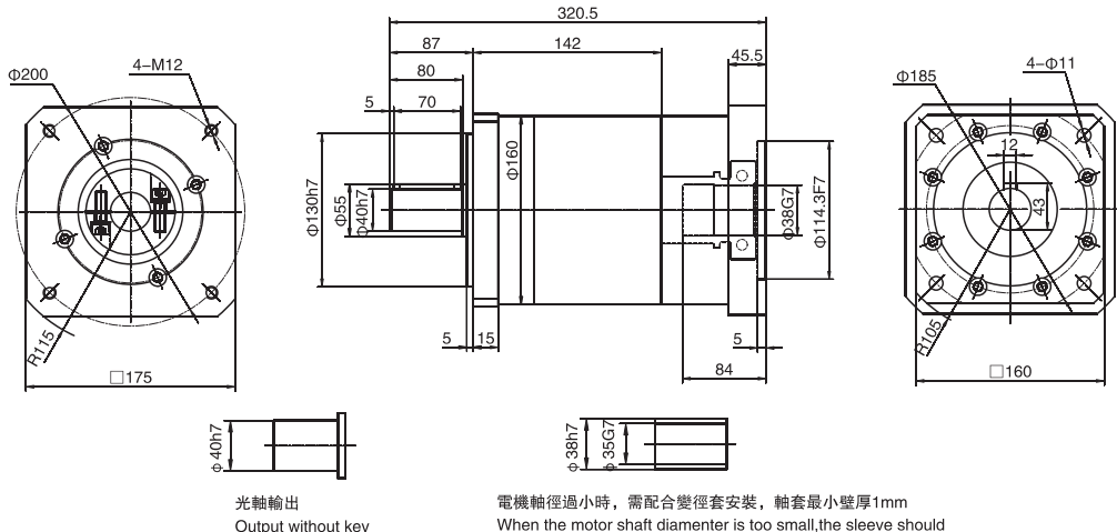
WPLF160雙級 / Double stage
