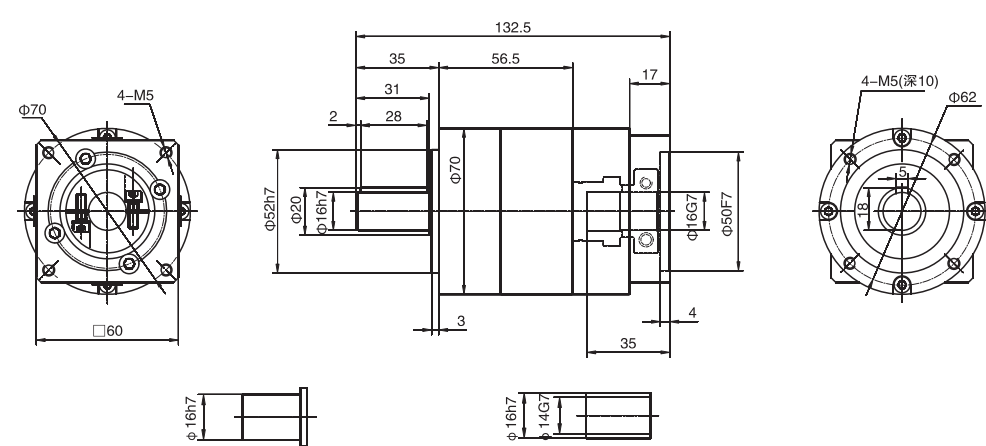
WPL70單級 / Single stage
