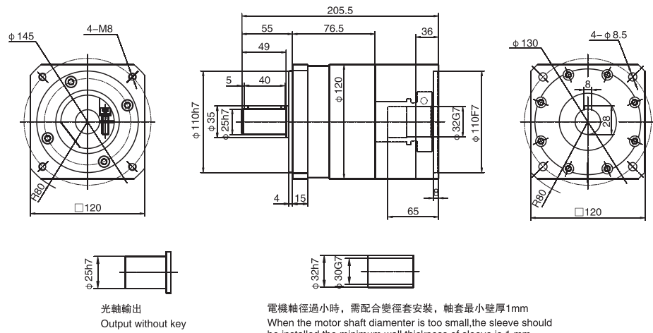
WPLF120雙級 / Double stage
