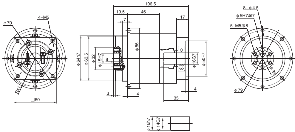
WPLH70單級 / Single stage
