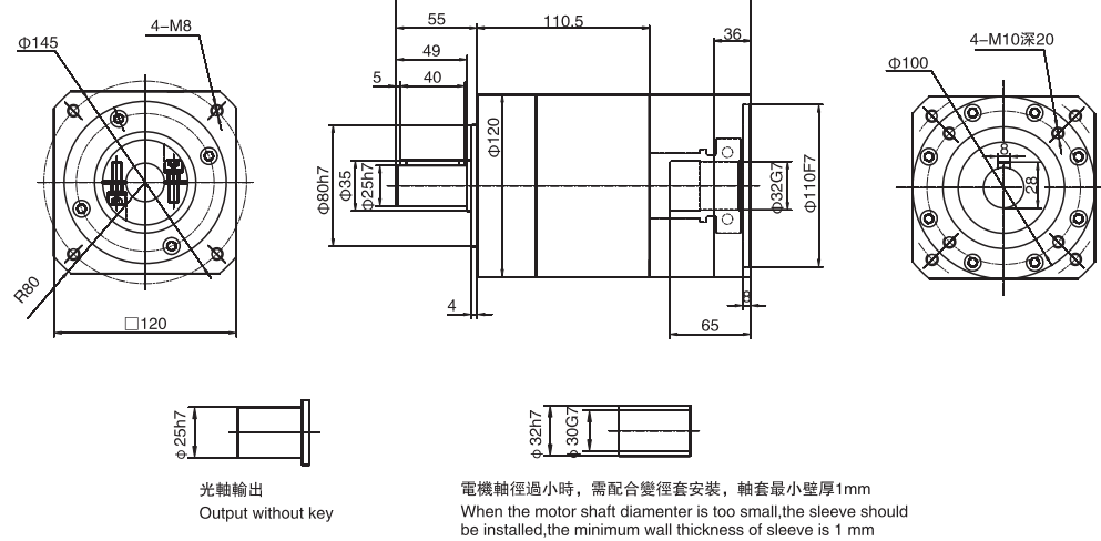
WPL120三級 / Three stage
