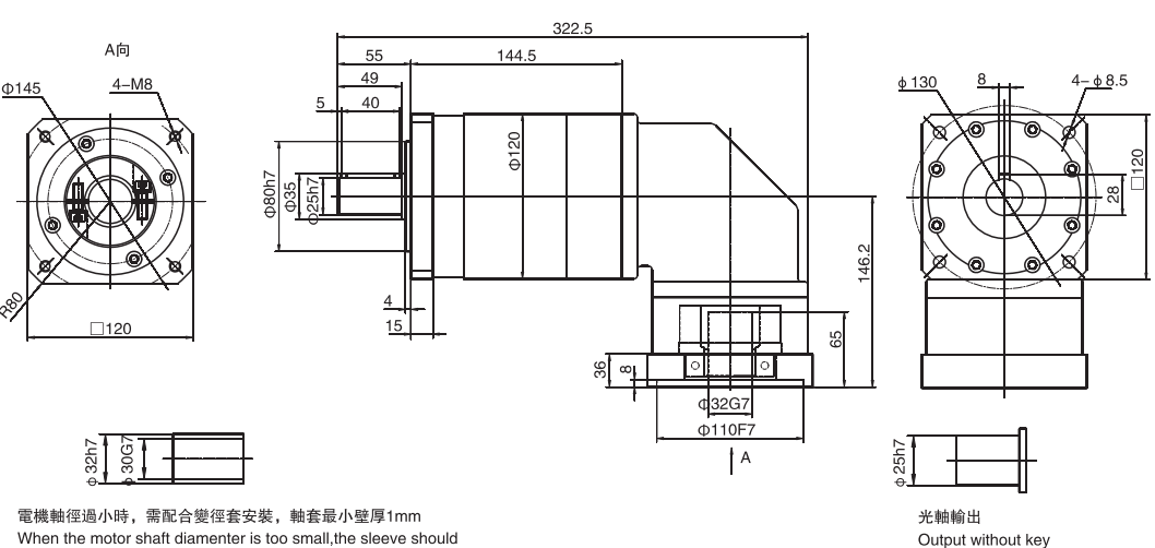
WPLFR120三級 / Three stage
