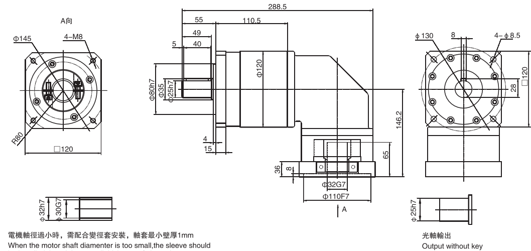
WPLFR120雙級 / Double stage
