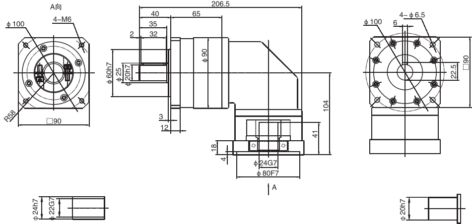
WPLFR90單級 / Single stage
