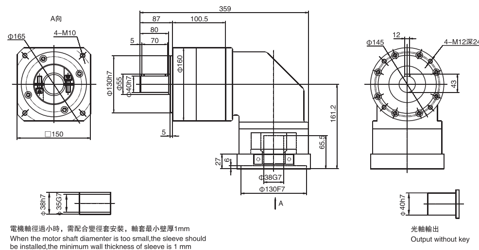
WPLR160單級 / Single stage
