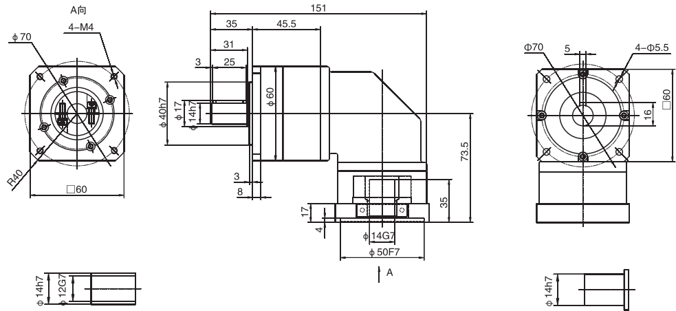
WPLFR60單級 / Single stage
