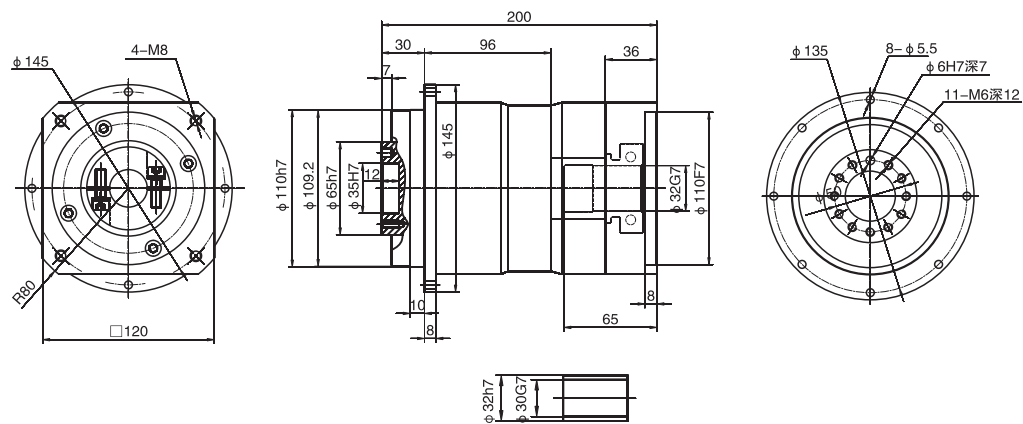
WPLH120雙級 / Double stage
