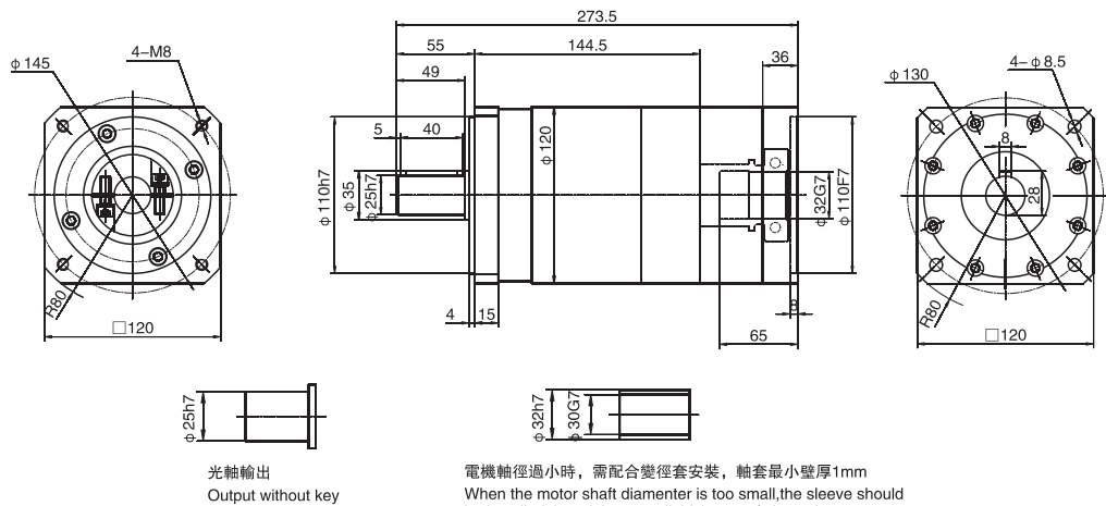
WPLF120三級 / Three stage
