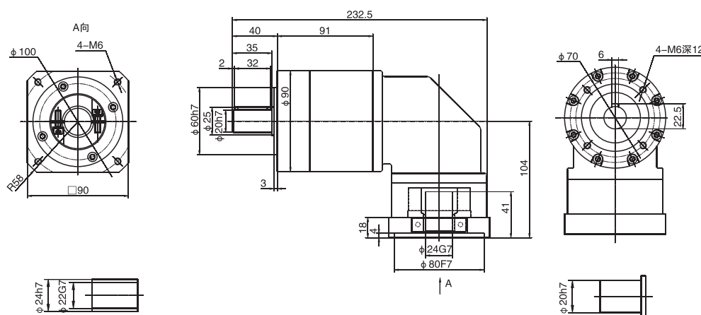
WPLR90雙級 / Double stage
