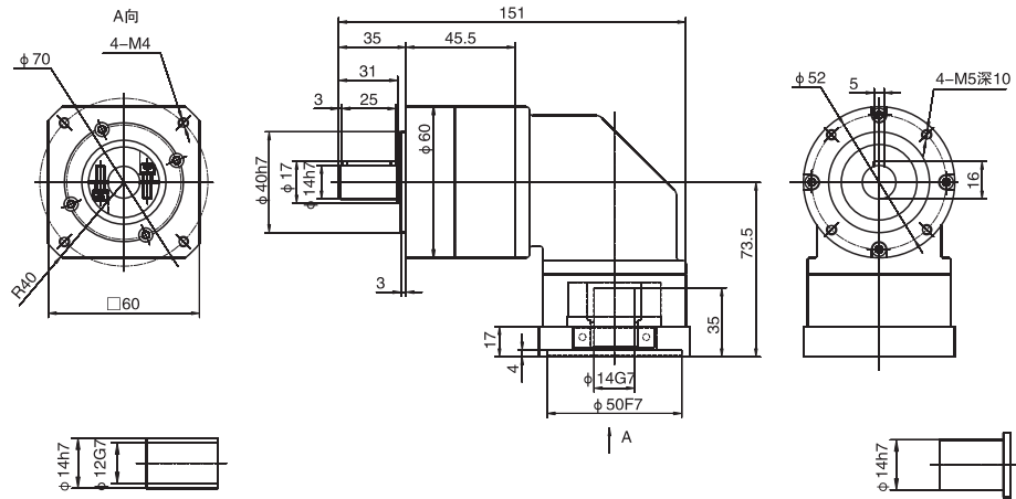
WPLR60單級 / Single stage
