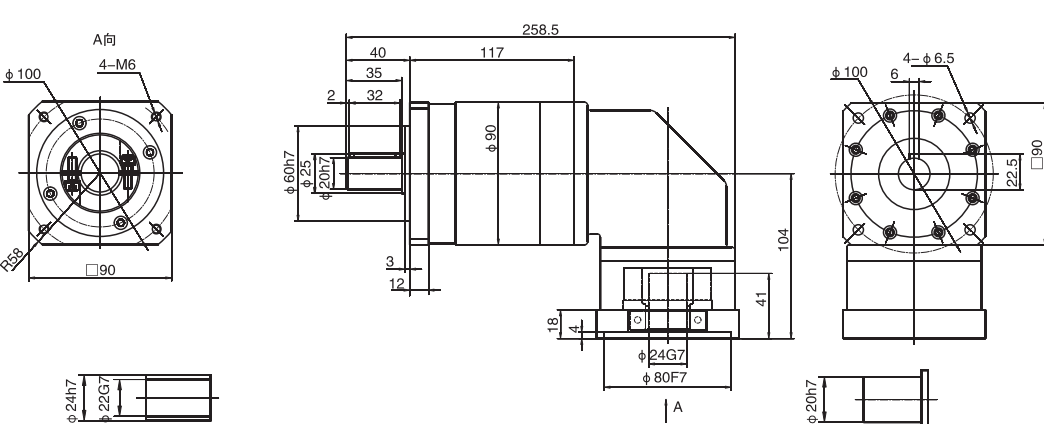
WPLFR90三級 / Three stage
