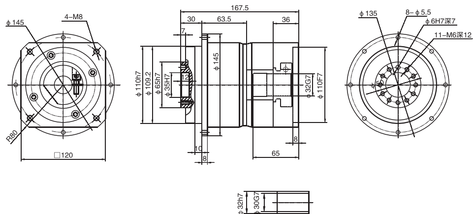
WPLH120單級 / Single stage
