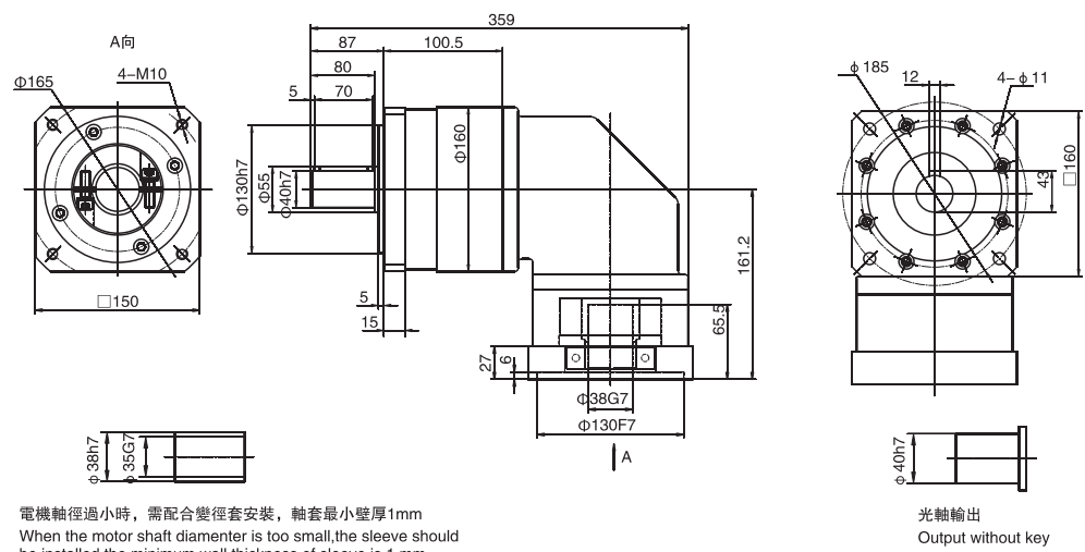
WPLFR160單級 / Single stage
