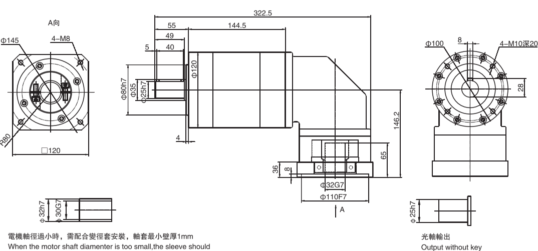
WPLR120三級 / Three stage
