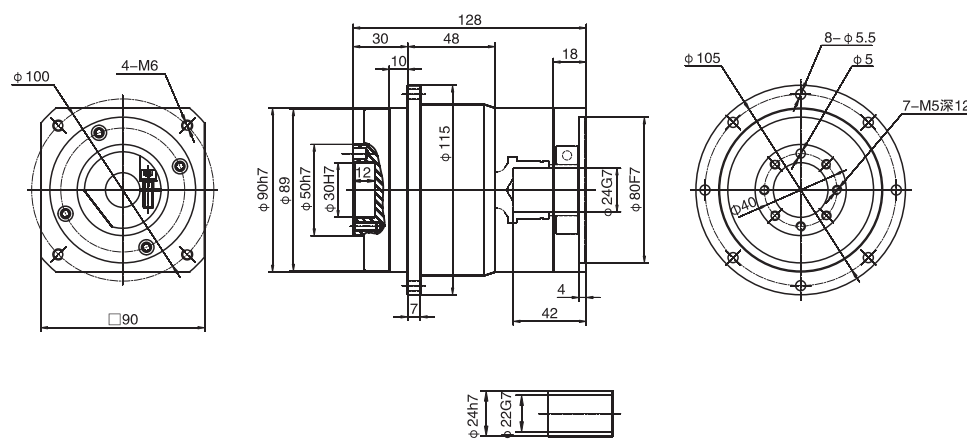
WPLH90單級 / Single stage
