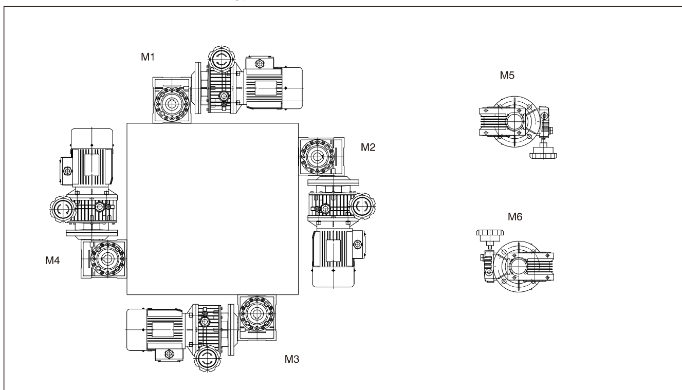
Mounting position of MB variator and WMRV series reducer
