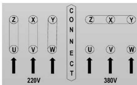
Connection diagram
