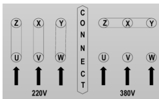
Connection diagram
