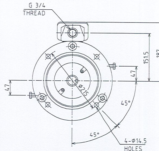
VIEW OF ARROW "A"
