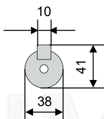
Output shaft
