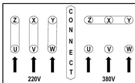
Connection diagram
