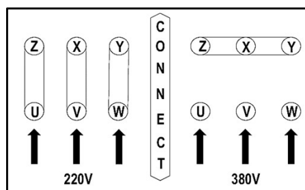
Connection diagram
