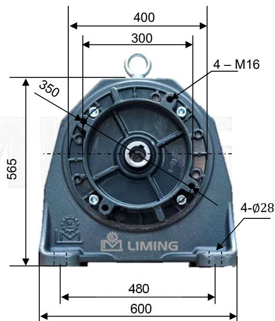
Output shaft
