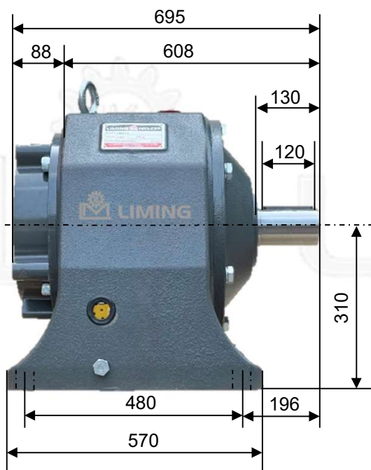
Output shaft
