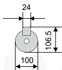
Output shaft
