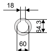
Input Bore
