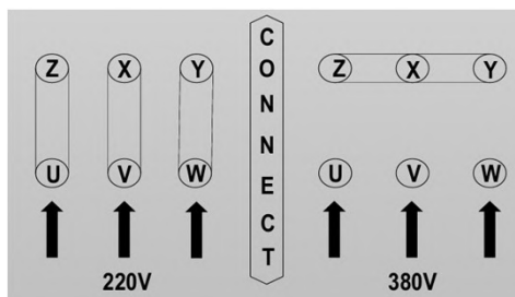
Connection diagram
