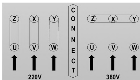
Connection diagram
