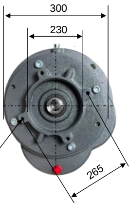
Input Bore
