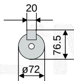
Output shaft
